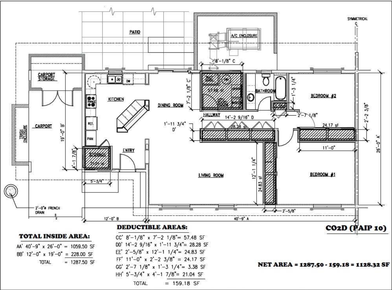
JUNIOR ENLISTED 2 BEDROOM - CO2D10
