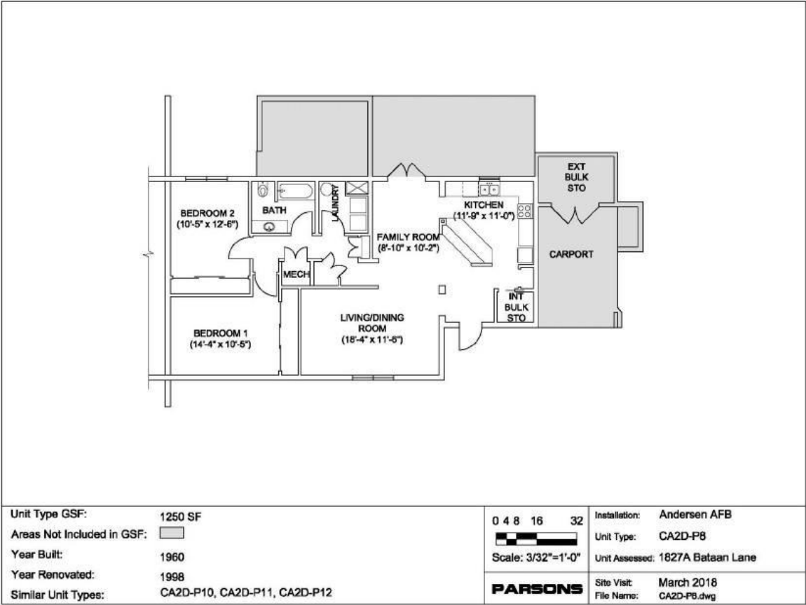
JUNIOR ENLISTED 2 BR - CA2D8/CA2D11/CA2D12
